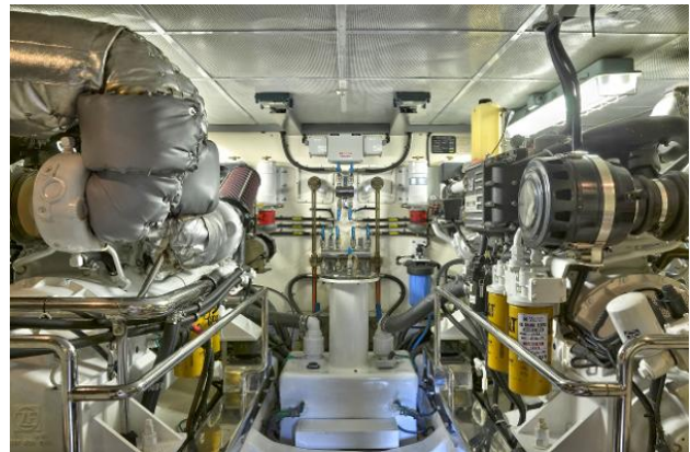
Engine Room
